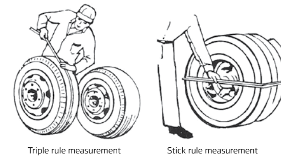
Measuring Circumference, diameter of dual-wheel tires
